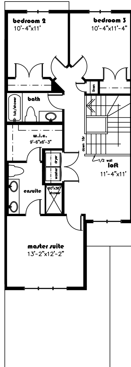
second floor 883
