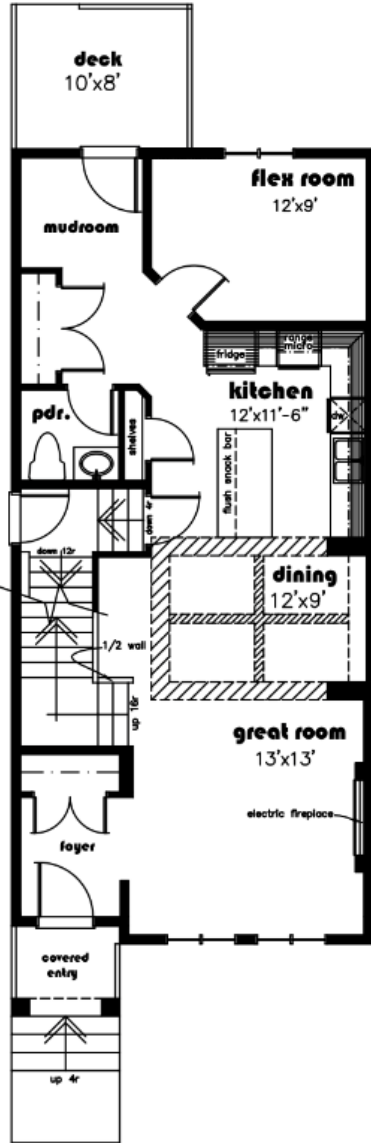
main floor 874 s.f.
